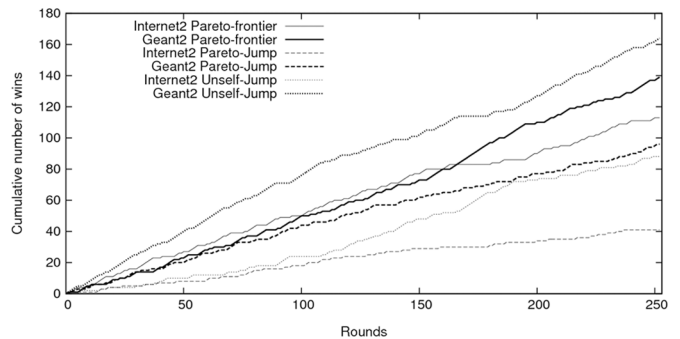
Fig. 8. Dynamics of the cumulative number of wins.
