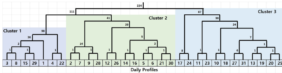
Fig. 6. An example of UPGMA clustering of profiles.
