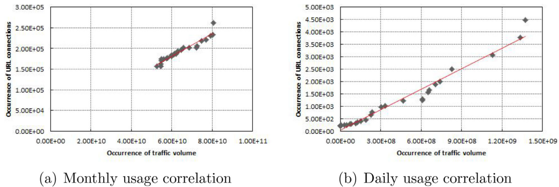
Fig. 1. Correlation of data volume and number of connections.
