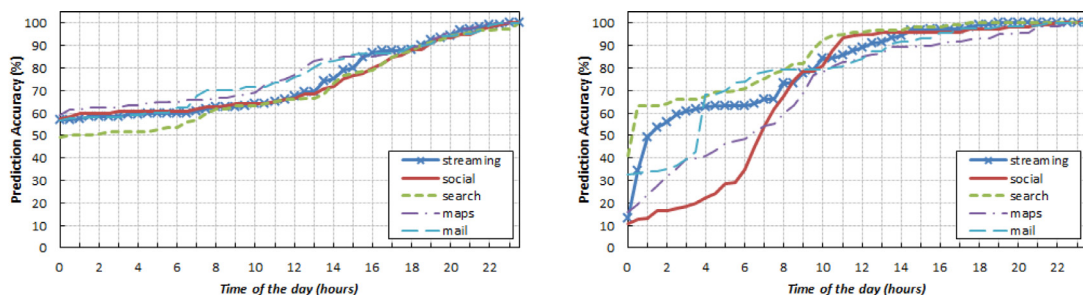
(a) Accuracy of 5 applications using 2-quantile (b) Accuracy of 5 applications using Student's test
