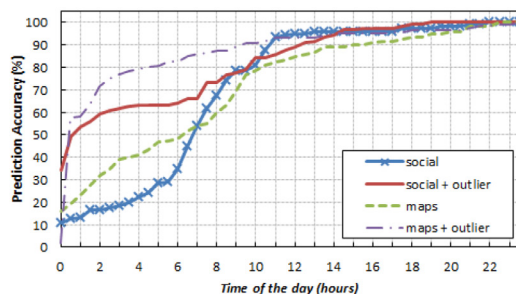
(a) Accuracy of Student's test with outlier detection
