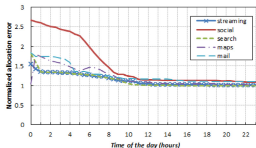
(c) Normalized allocation error of Student's test
