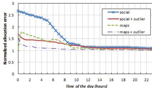
(b) Allocation error of Student's test with outlier detection
