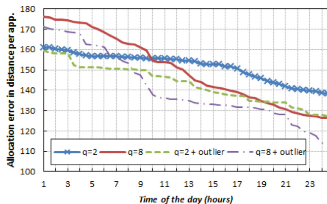
Fig. 12. Allocation error comparison using outlier detection.
