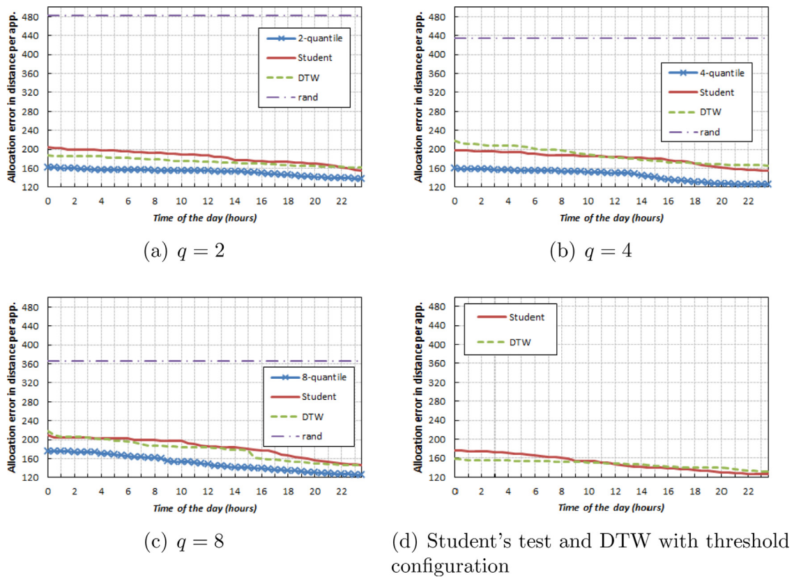
Fig. 9. Evaluation of allocation error.
