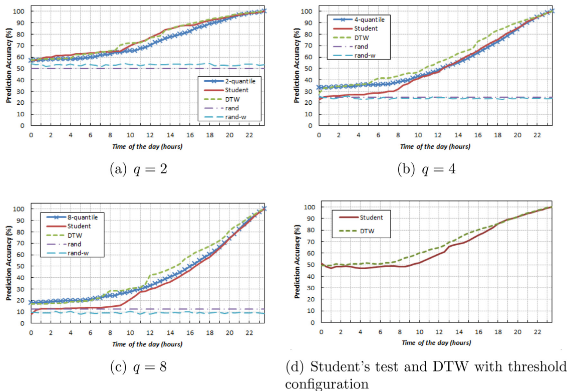
Fig. 8. Evaluation of prediction accuracy.
