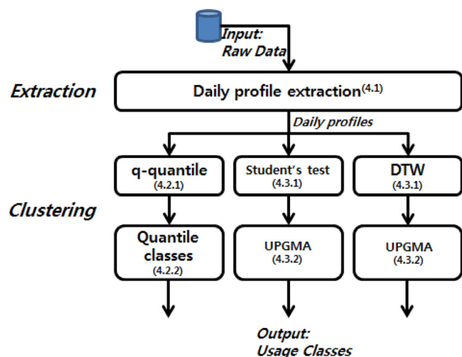
Fig. 3. Functional diagram of the proposed data clustering.
