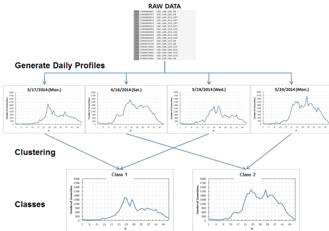
Fig. 4. Visual example of generating daily profiles and classes.
