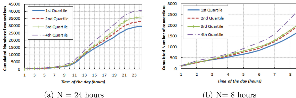
Fig. 5. Creation of classes using 4-quartile (quartile).
