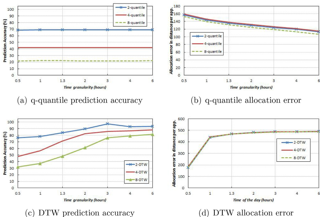
Fig. 10. Evaluation of time granularity.
