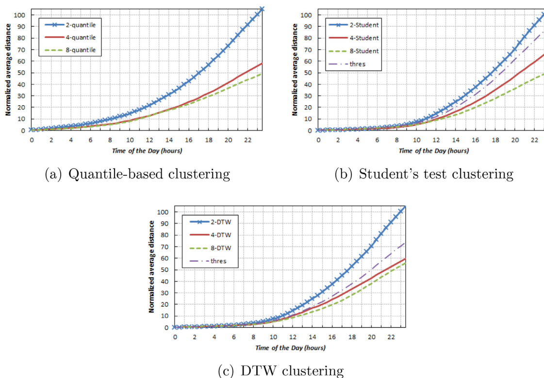
Fig. 7. Normalized average distance between classes.
