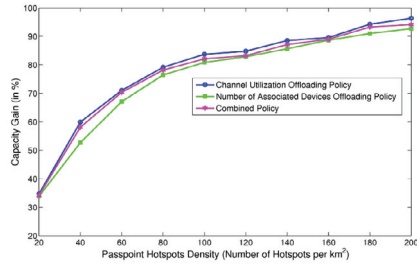
(a) Combination between Channel Utilization and Number of Associated Devices offloading policies
