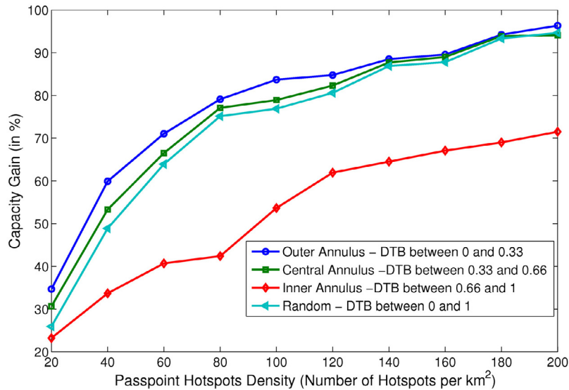
Fig. 11. Capacity gain for different hotspot placement schemes under the best hotspot selection policy.
