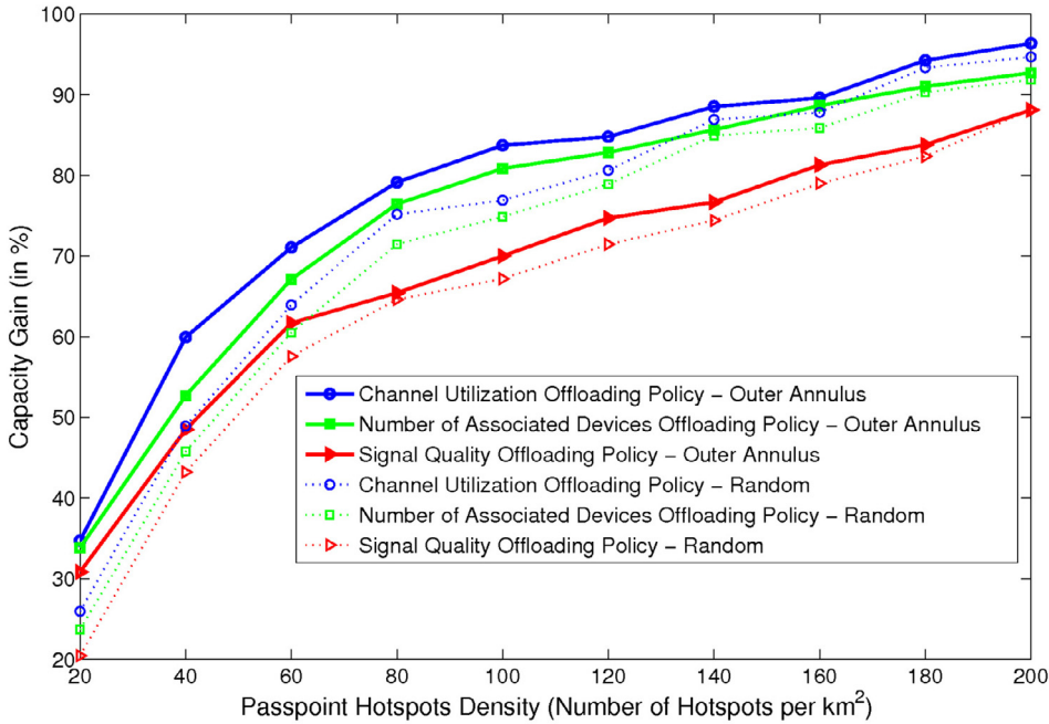
Fig. 12. Capacity gain for different Passpoint hotspot selection policies under the best placement scheme.
