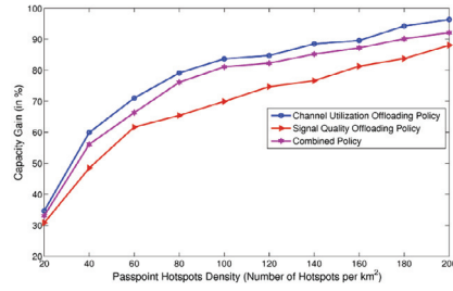
(b) Combination between Channel Utilization and Signal Quality offloading policies
