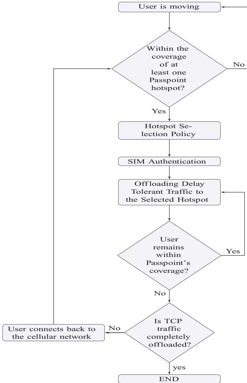
Fig. 5. Offloading algorithm.
