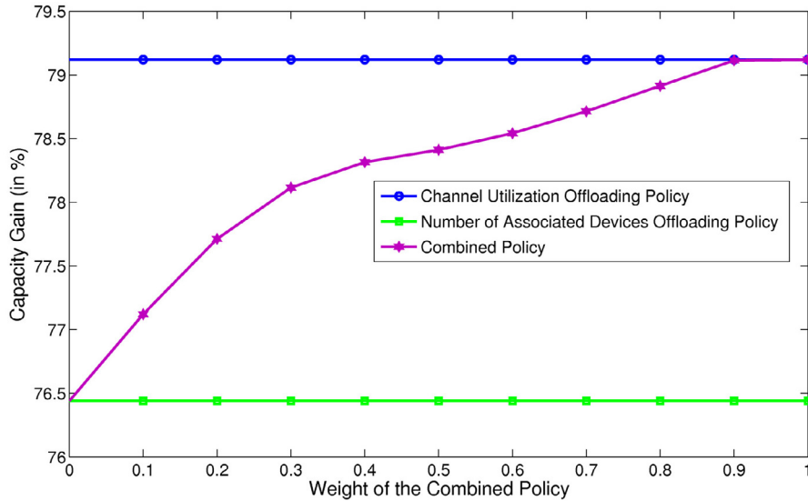
Fig. 14. Capacity gain for different weights under the best hotspot placement scheme (for a density of 80 hotspots/km 2 ).
