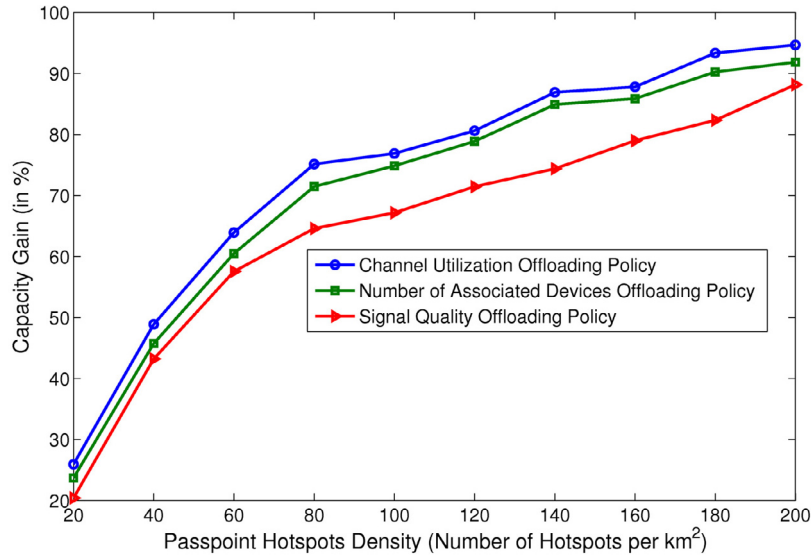
Fig. 6. Capacity gain for different Passpoint hotspot selection policies.
