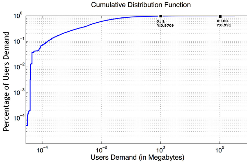
Fig. 4. Cumulative distribution function of users demands.
