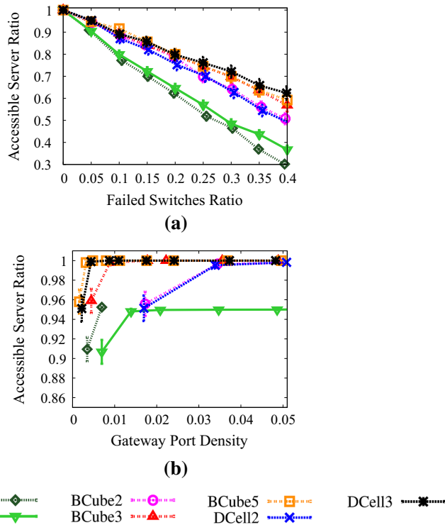
Fig. 15 GPD sensibility analysis in Survivable Phase for switch failures. a Accessible Server Ratio using minimum GPD, b ASR as function of the GPD for a Failed Switches Ratio of 0.05
